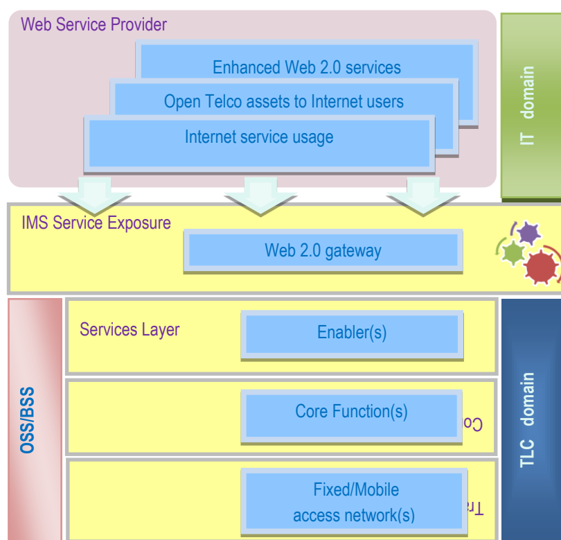
Figure 15: Platform architecture for NGN/IMS/web 2.0 service building.
