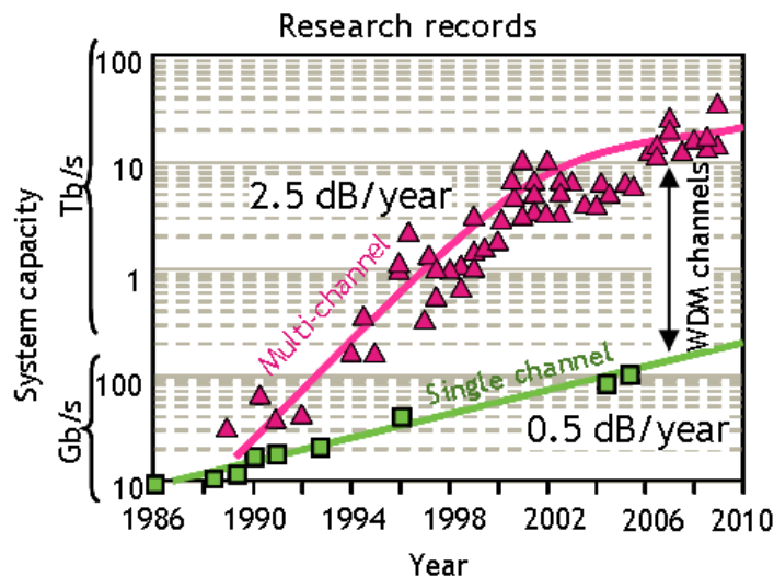
Figure 11: Evolution of the bit rate per optical channel and of the total capacity obtained thanks to WDM, transported through a single fibre (after S. Bigo, P. Winzer)
