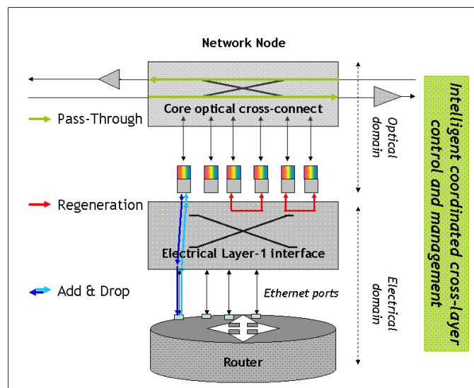
Figure 12: Intelligent cross-layer control and management for energy efficient network functions
